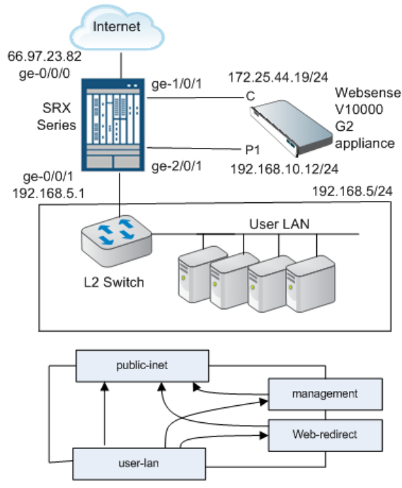
Figure 4: Example implementation network
