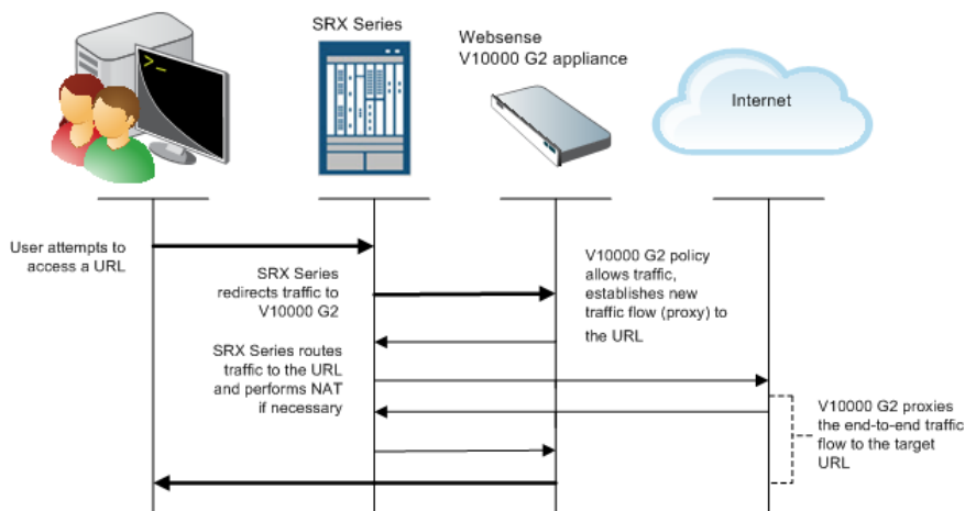
Figure 2: User traffic allowed
