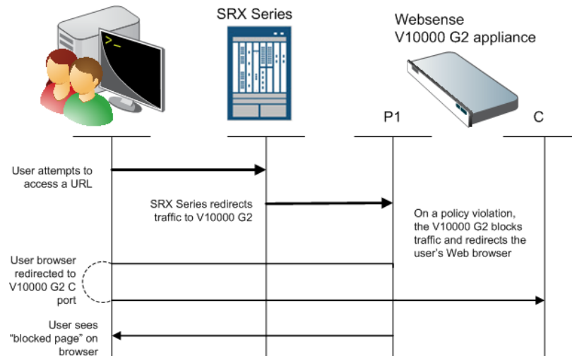
Figure 3: User traffic blocked
