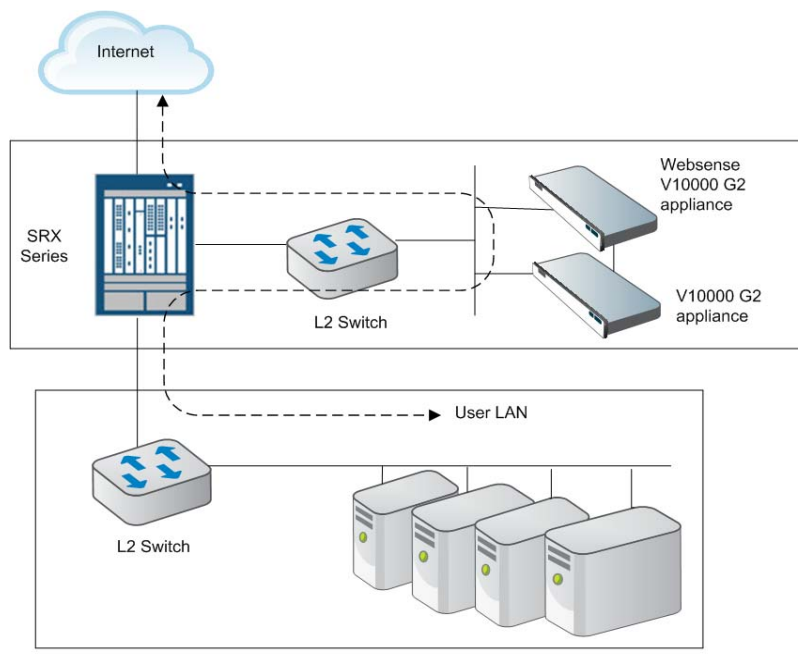
Figure 1: Reference network
