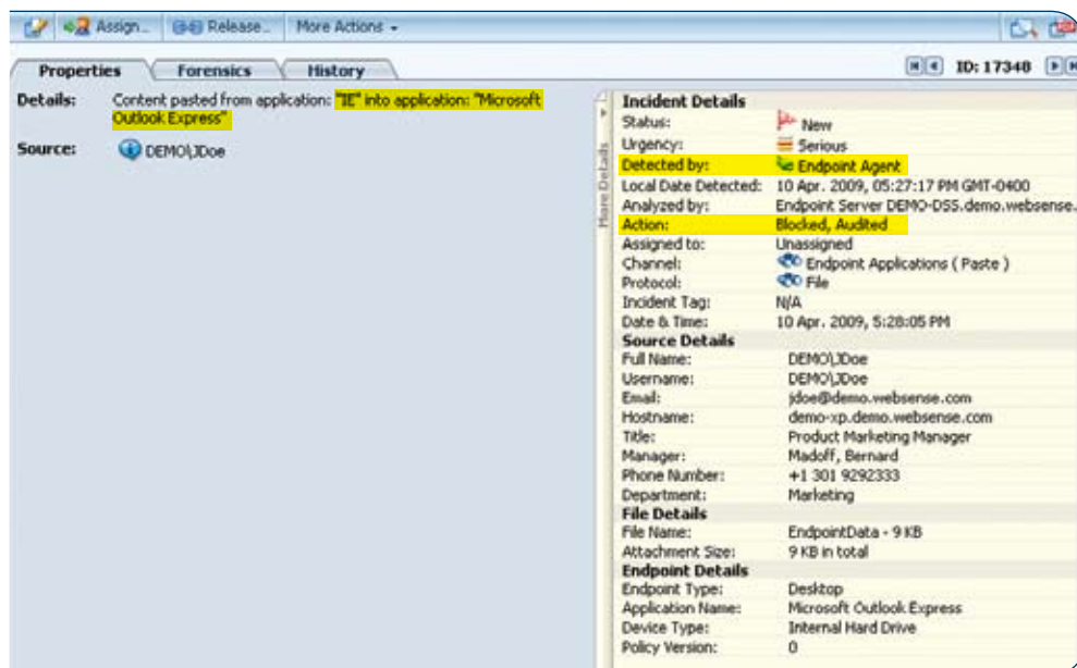
Incident detail with Websense Data Endpoint
